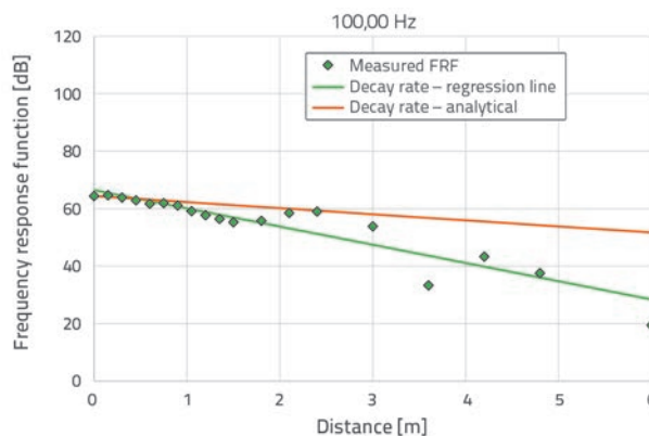
Figure 16. Frequency response function for one-third band around 100 Hz obtained during decay rate testing for standard track structure on ballast
