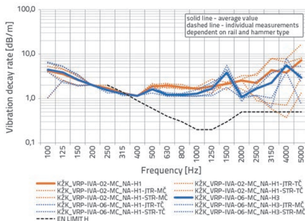
Figure 21. Comparison of decay rate in horizontal direction at two accelerometer positions (H1 and H3)
