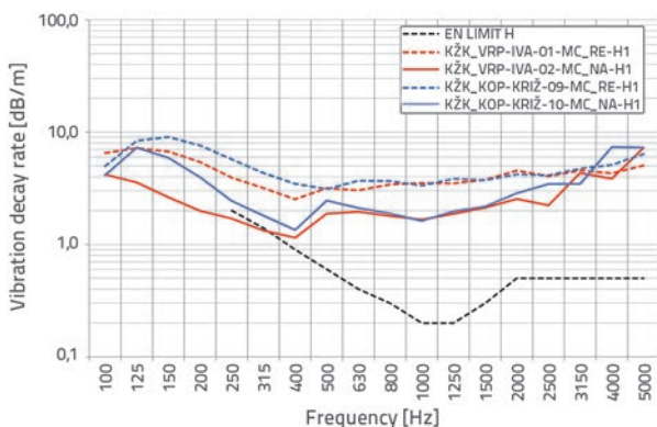
Figure 19. Comparison of methods for determining decay rate in horizontal direction
