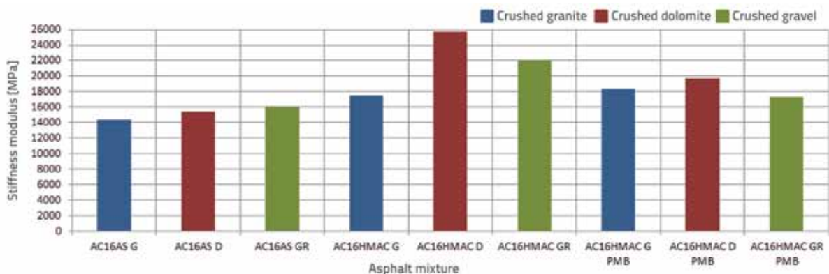
Figure 8. Distribution of stiffness modulus
