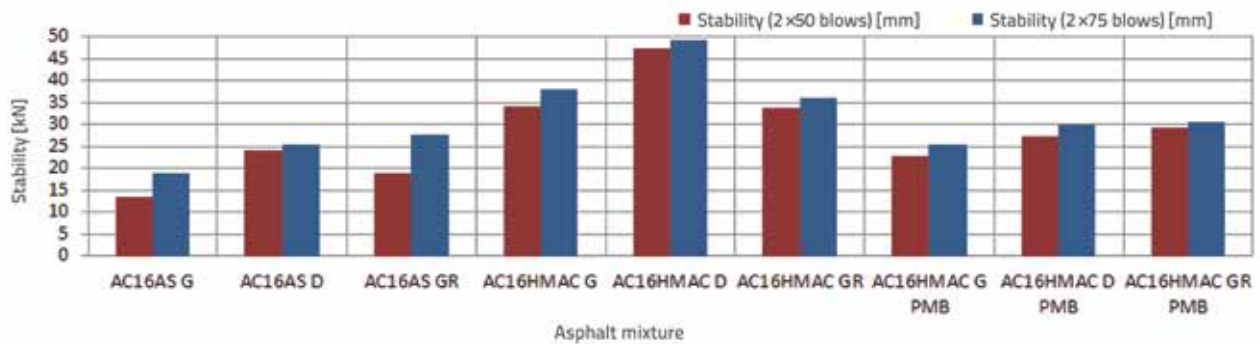
Figure 3. Distribution of Marshall stability
